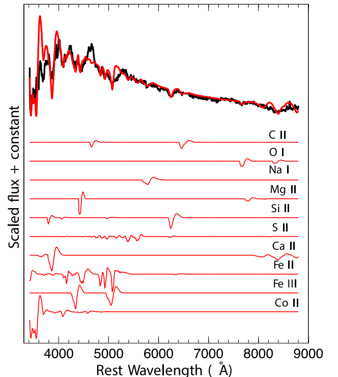
Figure 7. Optical spectrum of SN 2014ek taken at t \sim +1.8 days (black). The best-fitting SYNAPPS synthetic spectrum is overplotted. The contribution of each ion is shown in the lower part of the plot.
