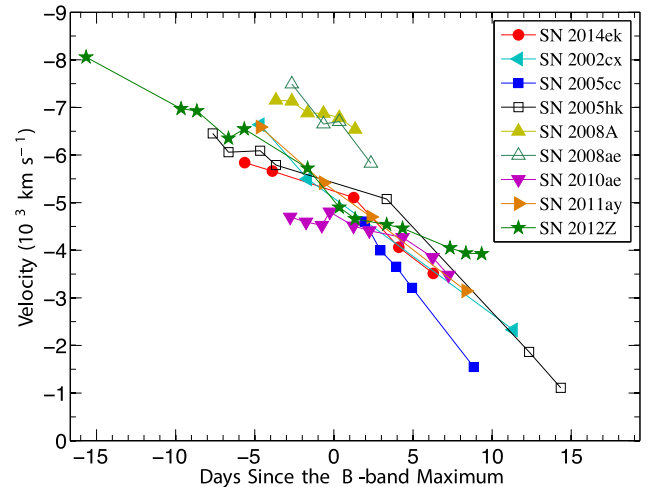
Figure 10. Comparison of velocity evolution of Si II \lambda 6355 between SN 2014ek and some other SNe Iax. Spectra of SN 2005cc are from Blondin et al. (2012), while references for the spectra of other SNe Iax are listed in the last column of Table 5.
