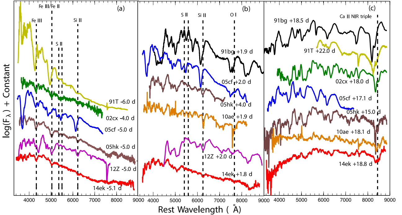
Figure 8. The spectra of SN 2014ek at t \sim -5.1, +1.8 and +18.8 days, compared with the spectra of SNe 2002cx (Li et al. 2003), 2005hk (Phillips et al. 2007), 2010ae (Stritzinger et al. 2014), 2012Z (Yamanaka et al. 2015), 2005cf (Wang et al. 2009), 1991T (Mazzali, Danziger & Turatto 1995) and 1991bg (Turatto et al. 1996) taken at similar phases. All spectra shown here have been corrected for the reddening of the Milky Way and redshift of the host galaxy.
