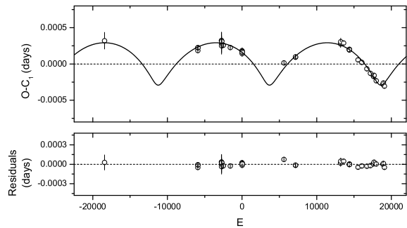
Figure 4. The theoretical light-travel time effect orbit of the circumbinary planet in RR Cae. After both the parabolic variation and the cyclic oscillation are subtracted, the residuals are displayed in the lower panel.
