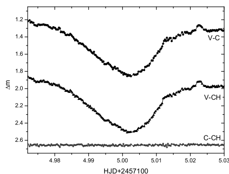
Figure 9. The eclipse profile of V363 Aur obtained with the 85-cm telescope in Xinglong observational station of national astronomical observatories (NAOs). "V" refers to V363 Aur, "C" to the comparison star, and "Ch" to the check star. Magnitude differences between V363 Aur, the comparison and the check stars are also shown in the figure.
