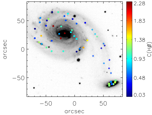
Fig. 3 The distribution of dust extinction c(H\beta) across Arp 86. The symbols are the same as in Fig. 1, where circles are from NGC 7753, squares from NGC 7752 and pluses from the bridge.
