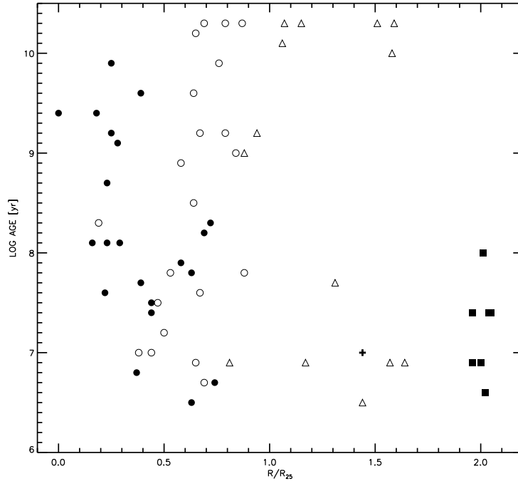
Fig. 7 Distribution of stellar ages in Arp 86. The ages are weighted by stellar luminosity (Cid Fernandes et al. 2005) and derived from spectral synthesis fitting. The filled symbols are the spectra with S/N \geq 3.0 (measured at 4730–4780 Å) and the open ones are the spectra with S/N < 3.0 (i.e., open circles are the regions in the galaxy NGC 7753, open triangles are the tidal bridge between the two galaxies).
