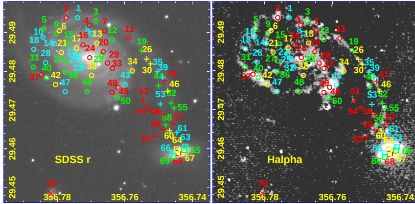
Fig. 1 Images of Arp 86, identifying the target H II regions. The background images are SDSS r (left) and H \alpha (right) images of Arp 86 with the target H II regions labeled. The symbols indicate the different data locations: circles – the dominant galaxy NGC 7753, squares – the companion galaxy NGC 7752, pluses – the tidal bridge between the two galaxies, and cross – the galaxy 2MASX J23470758+2926531. There are four colors and the targets with the same color were observed in the same mask. Region numbers are labeled in the figure and correspond to those given in Table 1.
